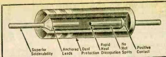
IRC TYPE GBT FIXED CARBON COMPOSITION RESISTORS
